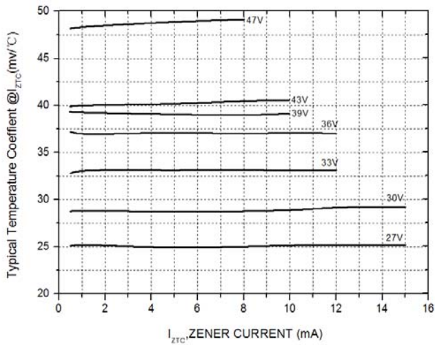
Fig 7: Typical Temperature Coefficient
