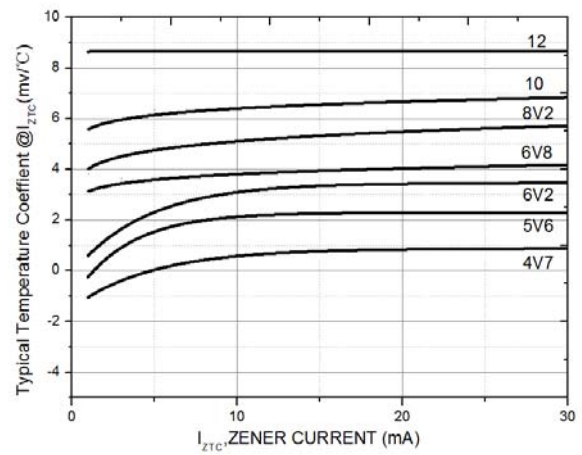
Fig 6: Typical Temperature Coefficient
