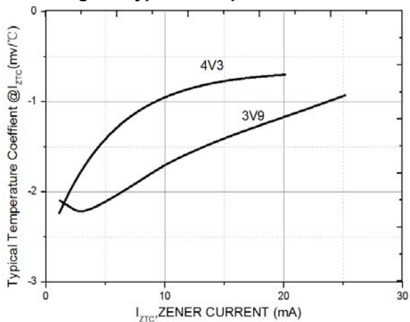
Fig 7: Typical Temperature Coefficient
